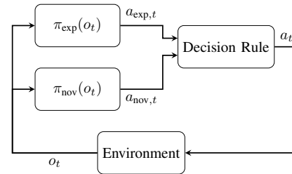
Fig. 2: Flowchart for DAgger variants, where the decision rule differs between approaches.
